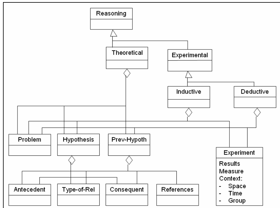
Figure 2: Class diagram of the Ontology for Scientific Knowledge in Articles
