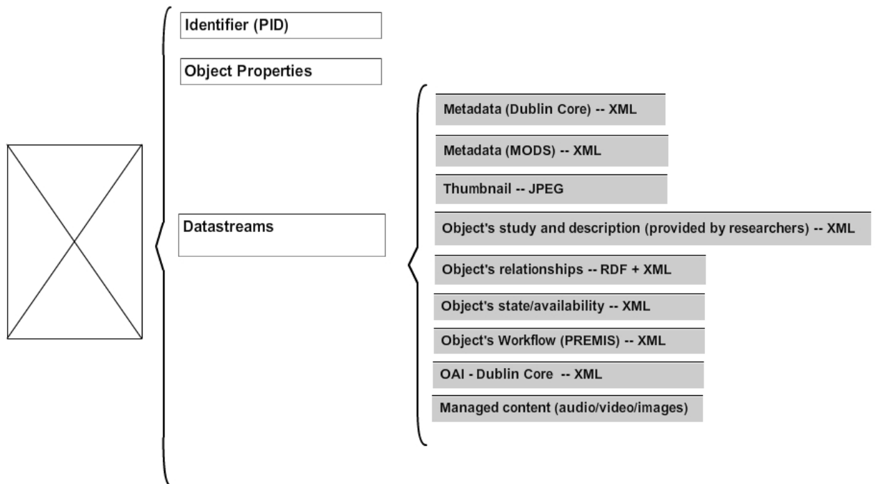
Fig. 2 Structure of a digital object in the repository
