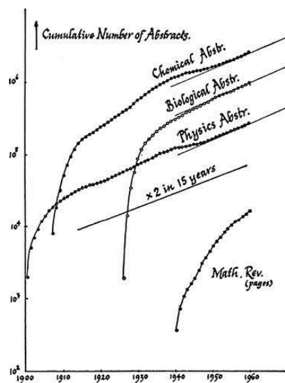
Fig. 2. CUMULATIVE NUMBER OF ABSTRACTS IN VARIOUS SCIENTIFIC FIELDS, FROM THE BEGINNING OF THE ABSTRACT SERVICE TO GIVEN DATE It will be noted that after an initial period of rapid expansion to a stable growth rate, the number of abstracts increases exponentially, doubling in approximately 15 years.
