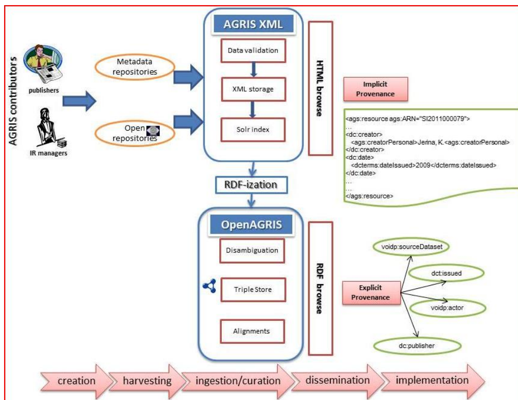
Fig. 1. Derivation history of an AGRIS artifact
